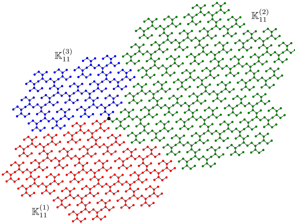
Figure 4. The set \mathbb{P}_{11} . In order to enlight the tree structure the point 0 is shown in black and adjacent points are connected.
